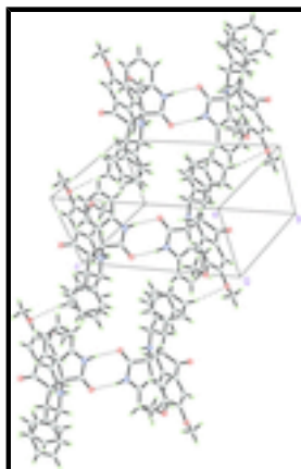
Fig. 2. The crystal packing of title compound, showing chains along the [110] direction. Intermolecular hydrogen bonds are shown as dashed lines.
